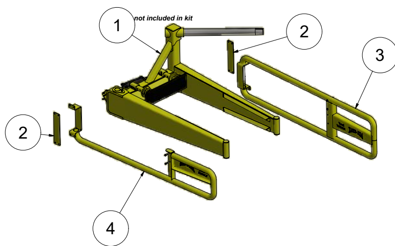
Bale Bundle Attachment Asm Part # 100669
