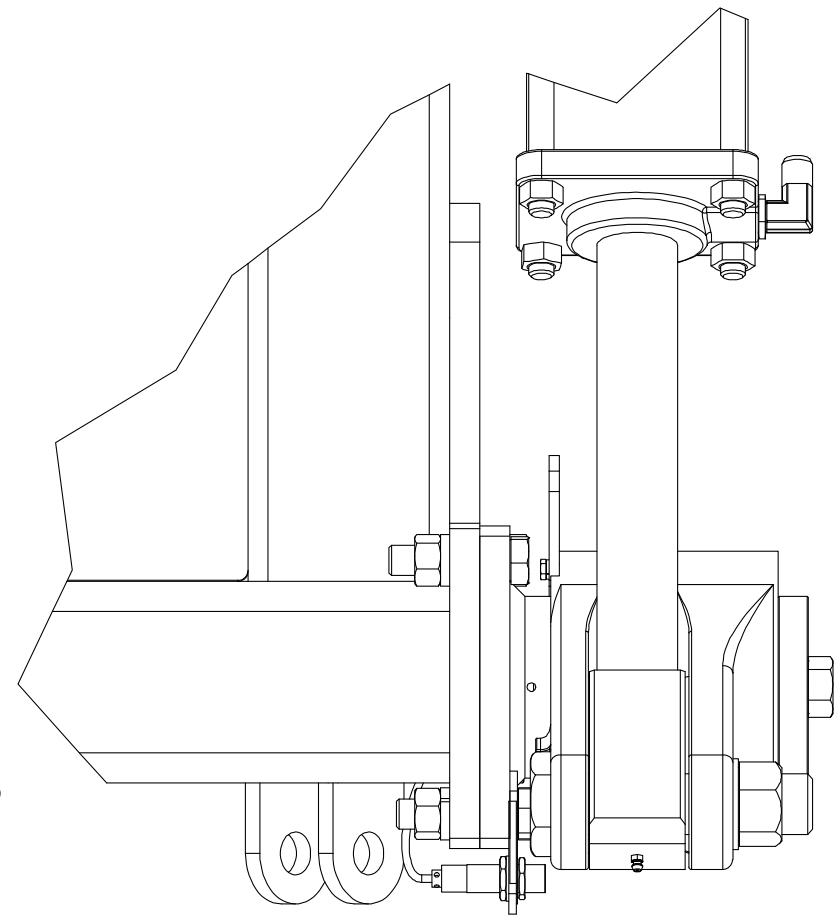
view A
